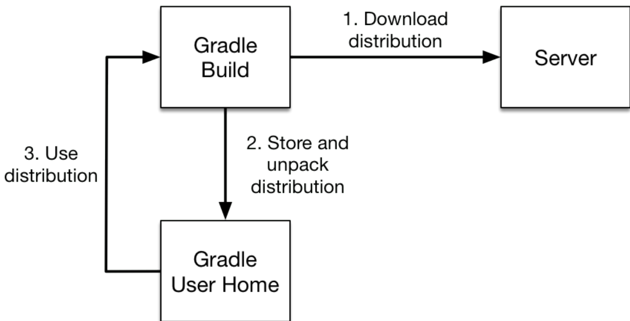
Figure 31. The Wrapper workflow
