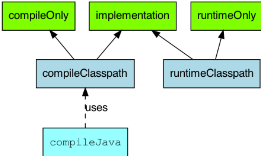
Figure 34. Java plugin - main source set dependency configurations
