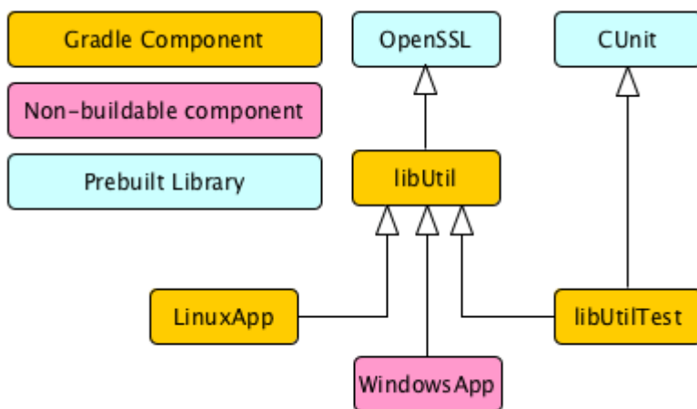
Figure 28. Dependent Components Example
