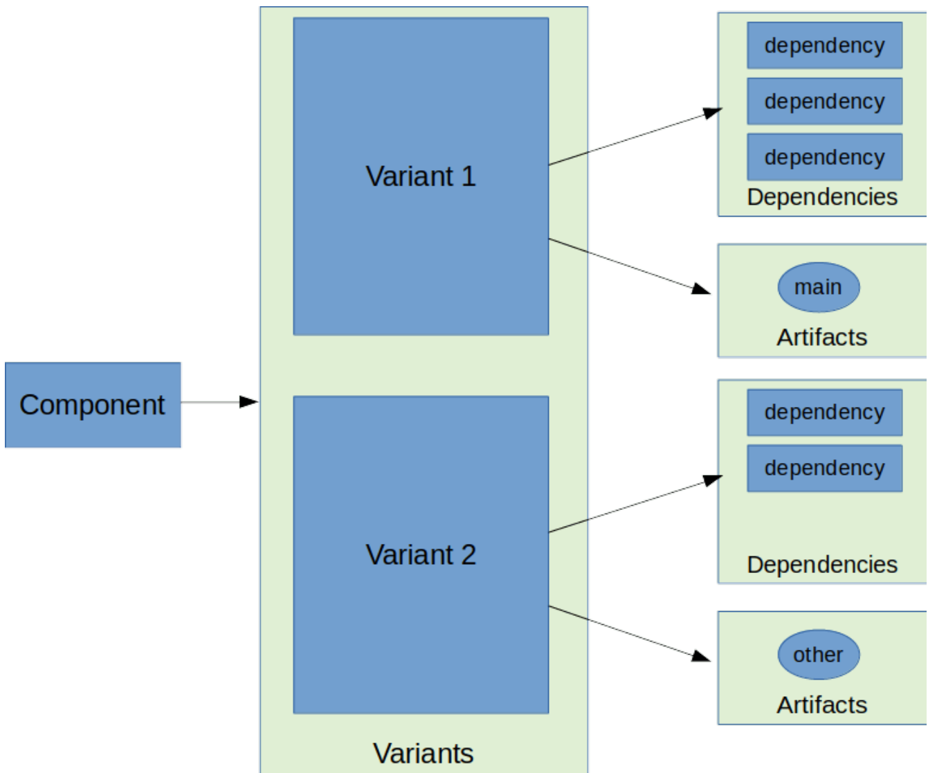
Figure 22. The Gradle component model
