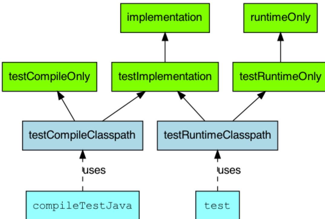
Figure 35. Java plugin - test source set dependency configurations
