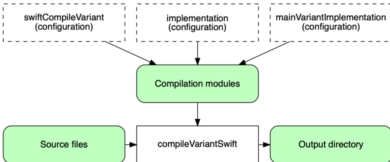
Figure 27. Sources and Swift compilation
