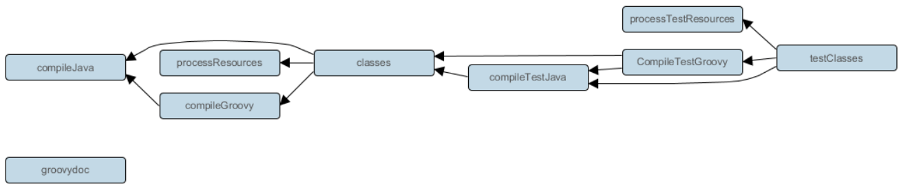
Figure 32. Groovy plugin - tasks
