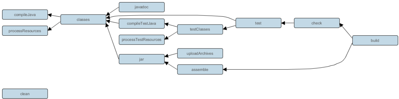
Figure 33. Java plugin - tasks
